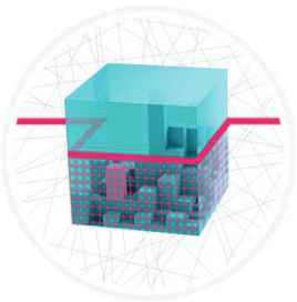
UEFI Scanner
