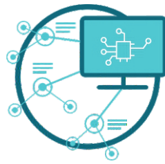
MACHINE LEARNING
