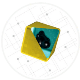
In-product Sandbox
